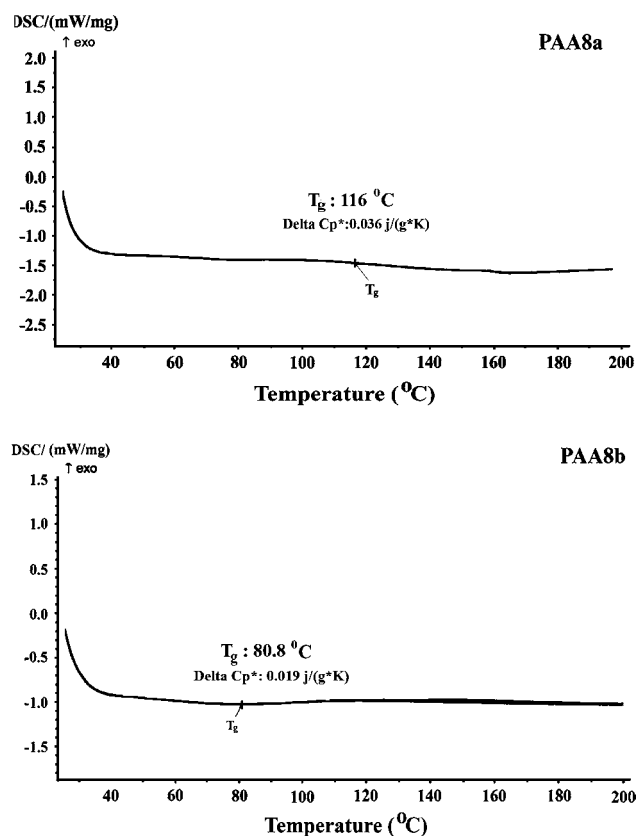
Fig. 5 DSC thermograms of PAA8a and PAA8b under N_2 atmosphere and a heating rate of 20^\circ\text{C min}^{-1}
